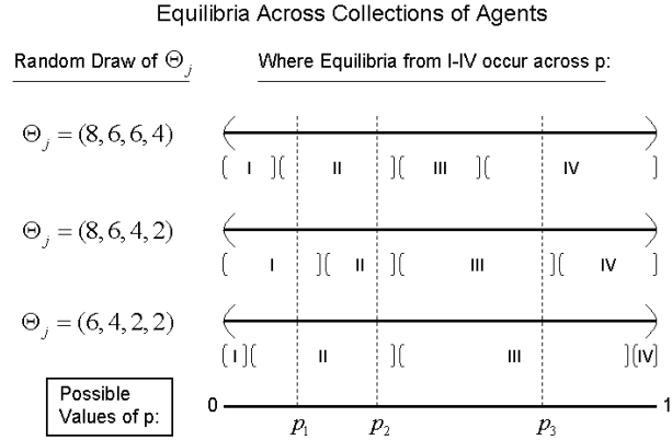
FIGURE 5.3. Location of Equilibria Over the Population.
