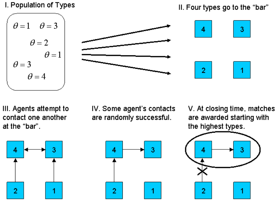
FIGURE 2.2. Steps of the Game for N = 4 , k = 1
