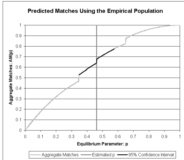
FIGURE 6.1. \hat{p} Estimate and Confidence Interval.
