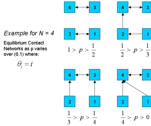
FIGURE C.1. Equilibria Across p in a four agent game.
